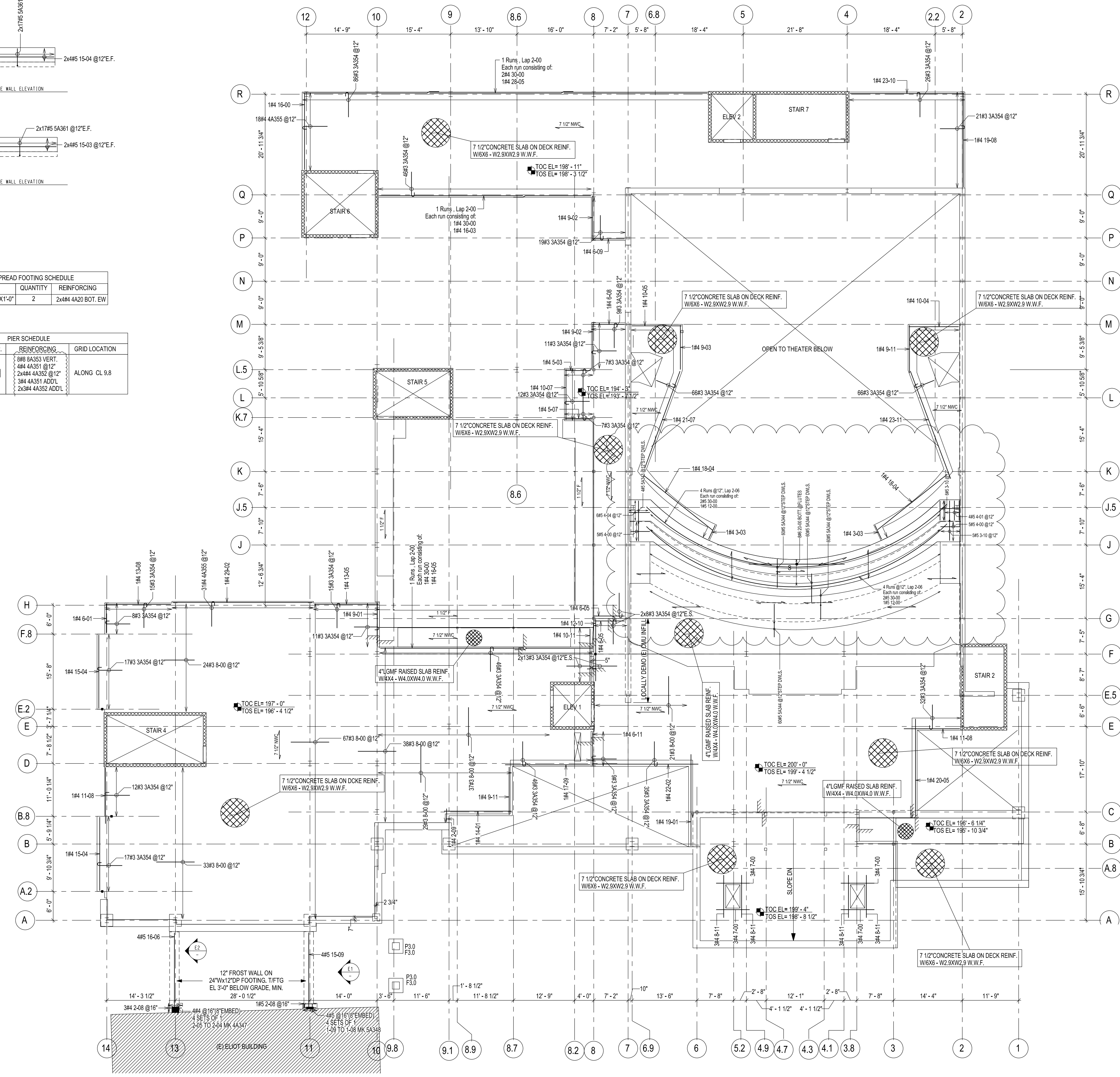
1 SLAB ON DECK PLAN - LEVEL 1 R200
